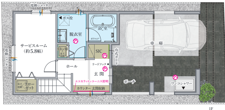
1F
